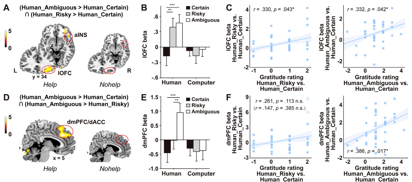
Fig. 4. Brain regions activated in the conjunction analysis. (A) Brain regions activated in [\text{Human\_Ambiguous} > \text{Human\_Certain}] \cap [\text{Human\_Risky} > \text{Human\_Certain}] , indicating the involvement of these regions in general-uncertainty-related processing. (B) Parameter estimates ( \beta values) corresponding to six conditions were extracted from right IOFC. Error bars indicate standard error of means. (C) The differences in IOFC activities between Human_Ambiguous and Human_Certain conditions ( r = 0.332, p = 0.042 ), and between Human_Risky and Human_Certain conditions ( r = 0.330, p = 0.043 ) were positive correlated with the differences in gratitude ratings between corresponding conditions. (D) Brain regions activated in [\text{Human\_Ambiguous} > \text{Human\_Certain}] \cap [\text{Human\_Ambiguous} > \text{Human\_Risky}] , indicating the involvement of these regions in ambiguity-sensitive processing. (E) Parameter estimates ( \beta values) corresponding to six conditions for dmPFC. (F) The differences in dmPFC activities between Human_Ambiguous and Human_Certain conditions ( r = 0.386, p = 0.017 ), but not Human_Risky and Human_Certain ( r = 0.261, p = 0.113 , taking out 2 outliers: r = 0.147, p = 0.385 ) were positive correlated with the differences in gratitude ratings between corresponding conditions. ^*p < 0.05 , ^{**}p < 0.01 , ^{***}p < 0.001 .
